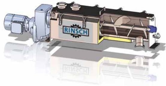
Beheizbare Mischschnecke Heatable Mixing Screw
